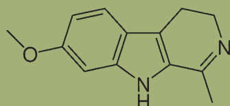
harmalin
